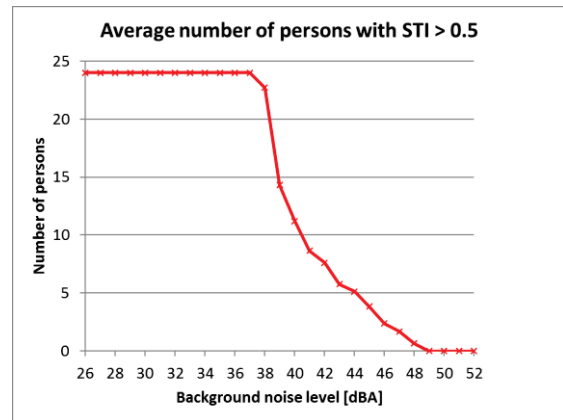
Figure 6: Average number of persons with STI above 0.5 for various background noise levels for the test room with acoustic ceiling (configuration b). This gives the average number of workers disturbed in their concentrated work by the speech signal of any one speaking coworker at a given background noise level.
