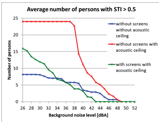
Figure 8: Average number of persons with STI above 0.5 for various background noise levels for the test room in three configurations.
