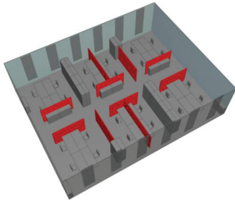
Figure 12: Office example two with 24 workplaces. The existing situation is displayed in gray. The absorbing screens to acoustically improve the situation are displayed in red.
