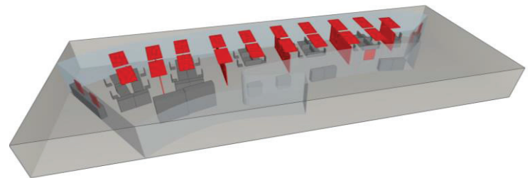
Figure 9: Office example one. elongated layout with 21 workplaces. The existing situation is displayed in gray. The measures to acoustically improve the situation are displayed in red: absorbing screens and absorbing elements at the wall and the ceilings.
