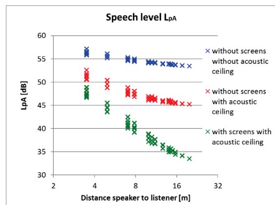
Figure 7: Graphic display of the speech levels for the test room in three configurations.
