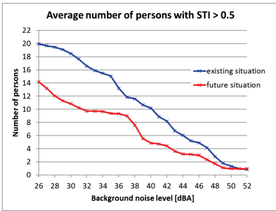
Figure 11: Average number of persons with STI above 0.5 for various background noise levels for office example one.
