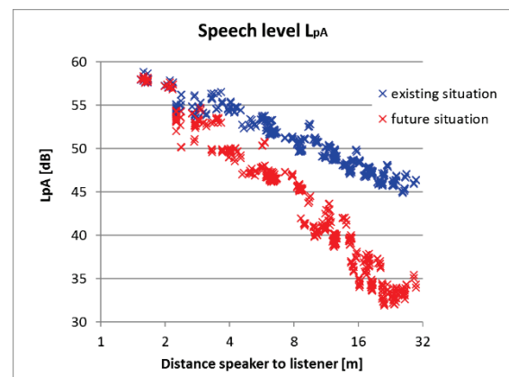
Figure 10: Graphic display of the speech levels for office example one.
