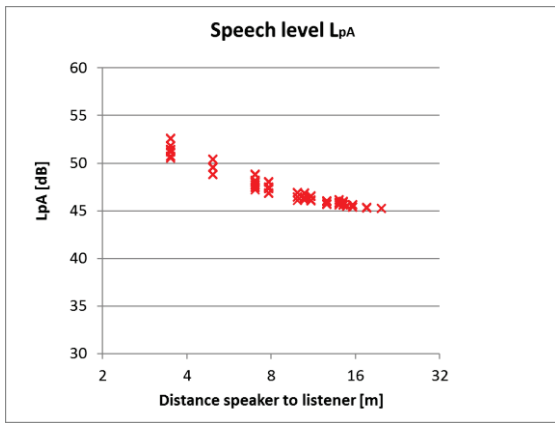
Figure 4: Graphic display of the speech levels for the test room with acoustic ceiling (configuration b) showing the speech levels as a function of the distance between speaker and listener.
