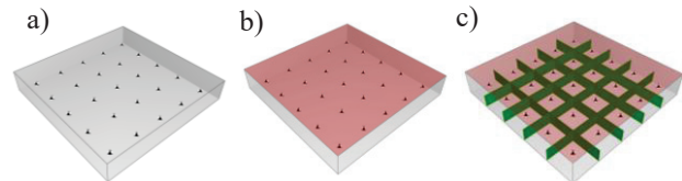
Figure 2: Configurations of the artificial test room: a) reverberant room, b) with acoustic ceiling, c) with acoustic ceiling and screens.
