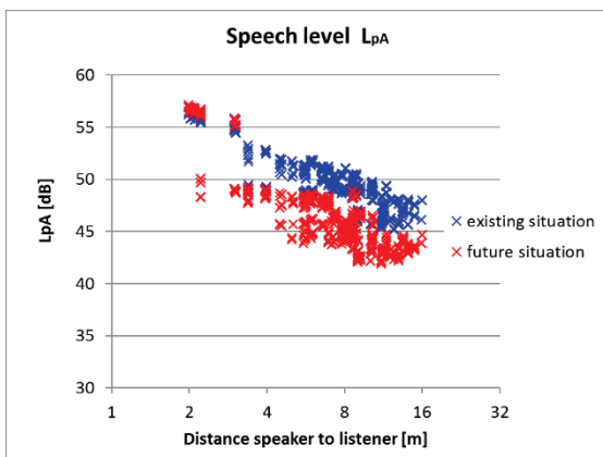
Figure 13: Graphic display of the speech levels for office example two.
