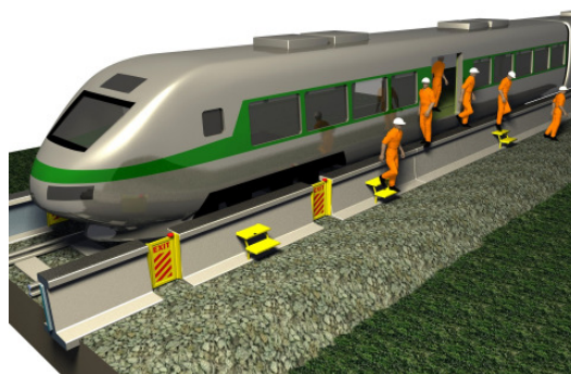
Figure 5.-Low barriers to screen the noise produced at the wheel-rail contact point
