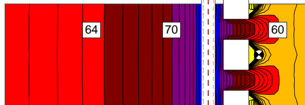
Figure 16 - NMPB 2008 homogene, refl. 1 st O., calculation time 1.2 second
