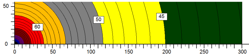
Figure 3 - NMPB 2008 homogeneous or favorable, reflecting ground ( G = 0 )
