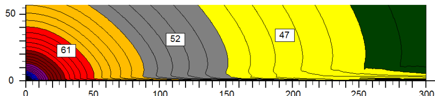
Figure 5 - Harmonoise Stability Class S5, reflecting ground ( G = 0 )
