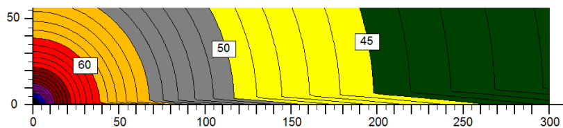
Figure 2 - ISO 9613-2, reflecting ground ( G = 0 )
