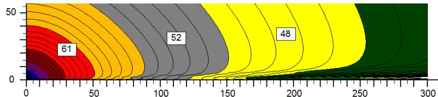
Figure 4 - Harmonoise Stability Class S1, reflecting ground ( G = 0 )
