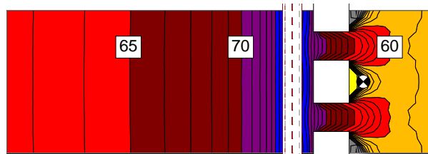
Figure 15 - ISO 9613-2*, refl. 1 st O., calculation time 1 second
