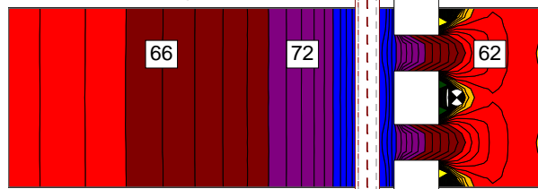
Figure 17 - Harmonoise S3, refl. 1 st O., calculation time 54.2 second
