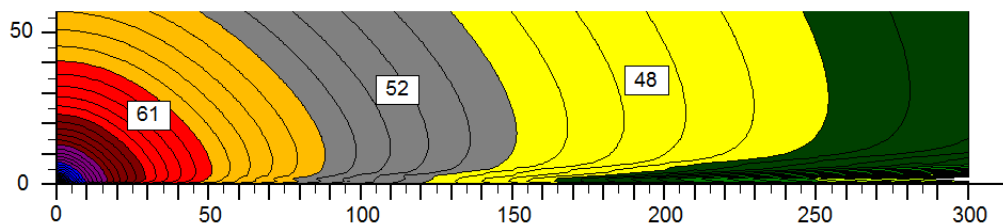
Figure 4. Harmonic Stability Class S1, reflecting ground ( G = 0 ).
