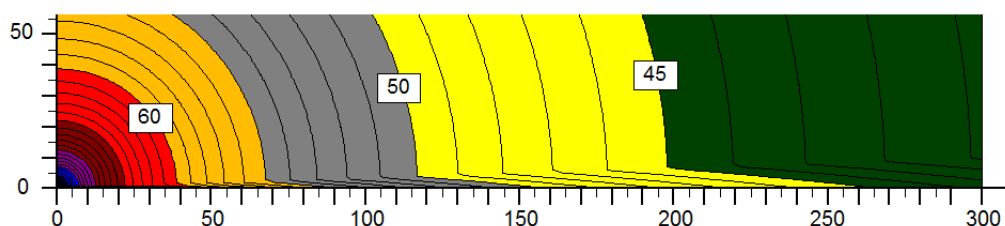
Figure 2. ISO 9613-2, reflecting ground (G = 0).
