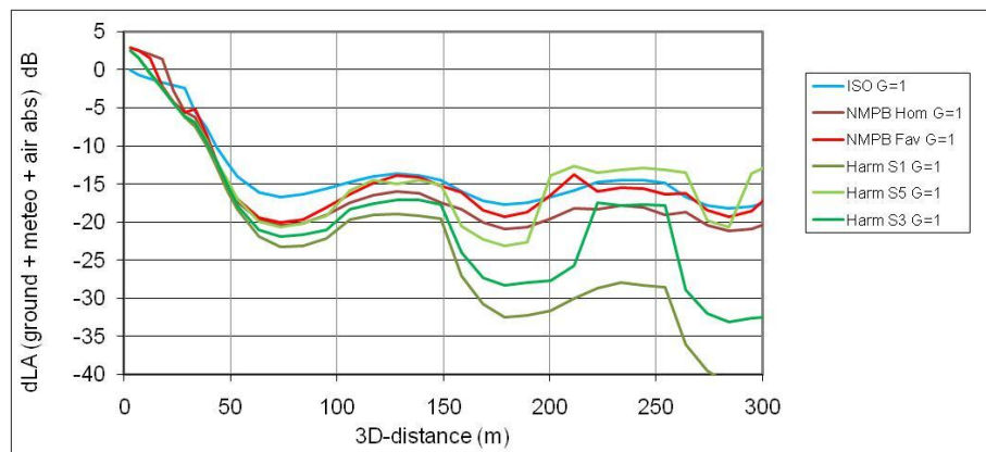
Figure 13. Normalized levels versus 3d-distance with porous ground ( G = 1 , 200 kRayl)
