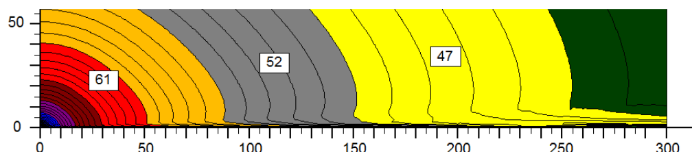
Figure 5. Harmonic Stability Class S5, reflecting ground ( G = 0 ).
