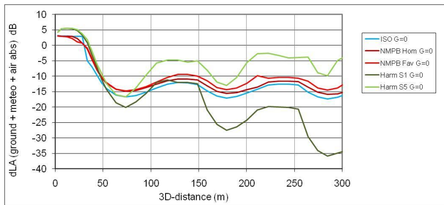
Figure 12. Normalized levels versus 3d-distance with reflecting ground ( G = 0 , 20000 kRayl)
