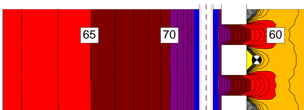
Fig. 15. ISO 9613-2*, refl. 1 st O., calculation time 1 second
