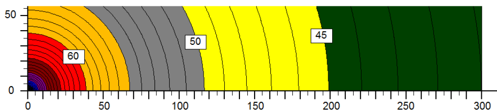
Figure 3. NMPB 2008 homogeneous or favorable, reflecting ground ( G = 0 ).
